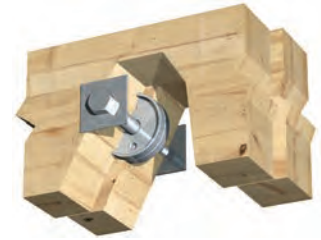
Shear Plate 67
