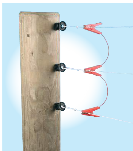
Fence connection cable with spring-loaded clamps (SS) provides optimum cross-connections for temporary polywire fences.
