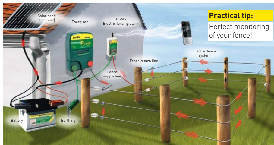
Schematic showing the monitoring of an electric fence system powered by batteries (with an optional solar panel) – within minutes the electric fence alarm will be transmitted from the most remote paddock to the mobile and/or landline telephone.
