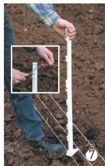
7 Put in the plastic posts and attach the polywires
