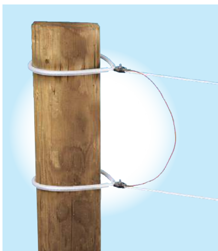
Fence connection cable - polyrope - with (SS) polyrope clamp provides optimum cross-connections for temporary polyrope fences.
