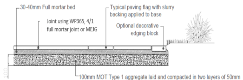
1 Typical section through a patio constructed in accordance with Marshalls Register Installation Procedures D01 Scale 1:20 @ A3
