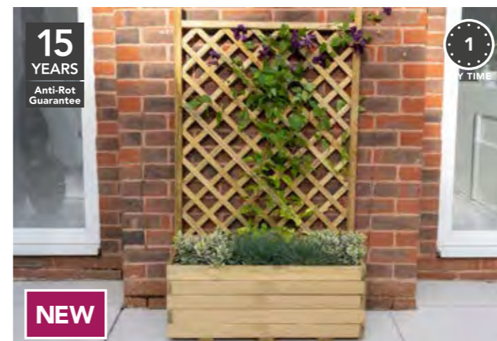
TRELLIS PLANTER TPLA(HD) (holds approx. 94L compost) 137(h) x 80(w) x 40(d)cm
