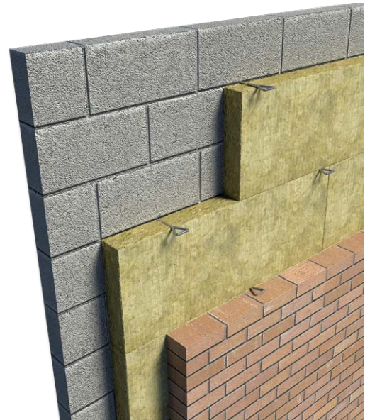
Figure 1 Wall tie positioning
