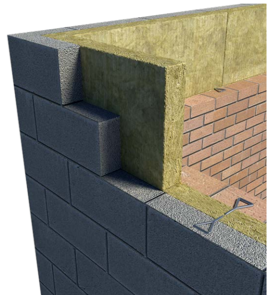
Figure 3 Slabs at corner detail
