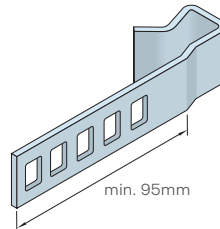
Hammer-On Section Lengths 95mm, 155mm, 215mm
