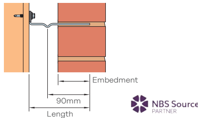
Ancon SDB Frame Cramp Fixed to Steel with Ancon Self-Drilling Screw
