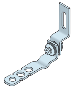
Ancon ACOU SD-ZV Frame cramp with integral drip and 8mm x 30mm fixing slot Suits 100-175mm cavities
