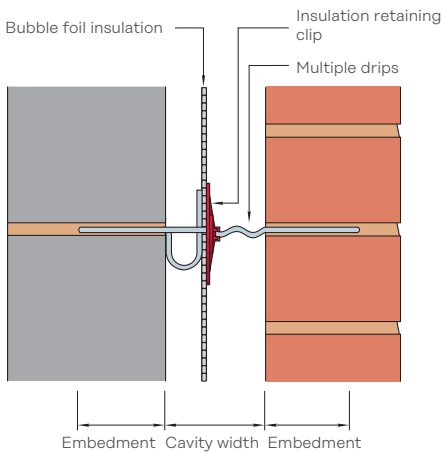
Installation of Ancon Staifix WT2-AF Wall Ties
