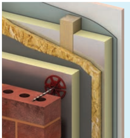
Ancon Staifix-Thor Helical TIM6 Tie
