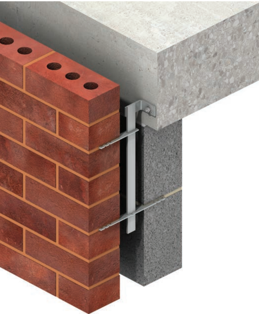
Ancon FHR Head Restraint - other sizes available
