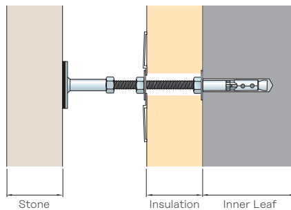
Ancon Push-Off Bolt
