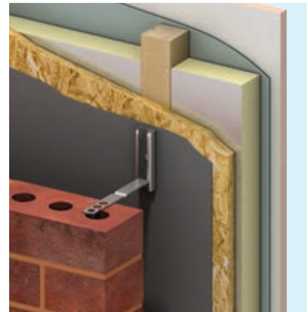
Ancon TFMT7 Timber Frame Movement Tie
