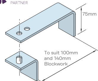
Ancon FHR Head Restraint - other sizes available
