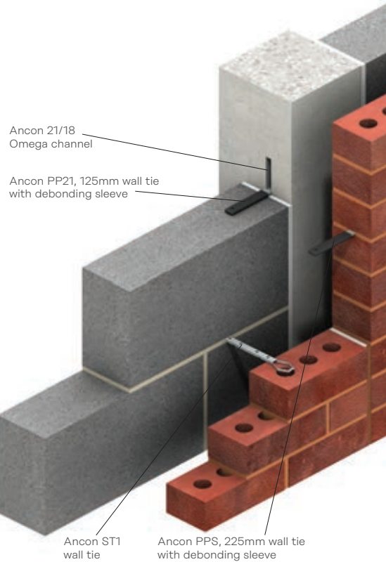
Intermediate Column with Vertical Movement Joint in Brickwork and Blockwork
