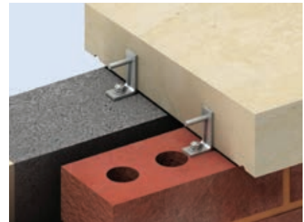
Two Ancon YPB Ties Restraining Coping Stone
