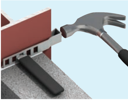
Ancon Hammer-On Tie
