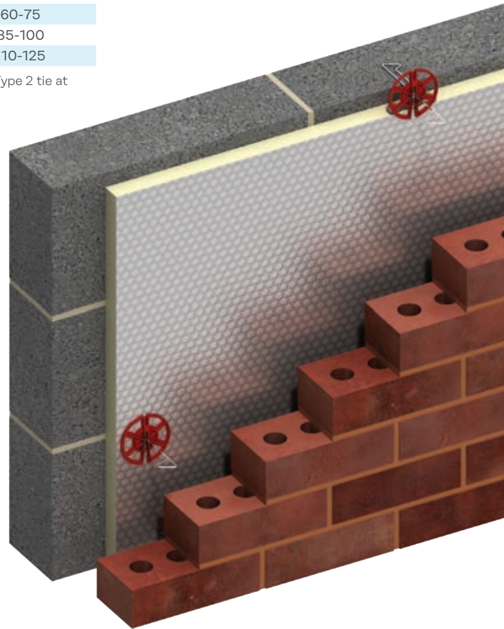
Ancon Staifix WT2-CB Wall Ties shown with Alreflex Ultratherm
