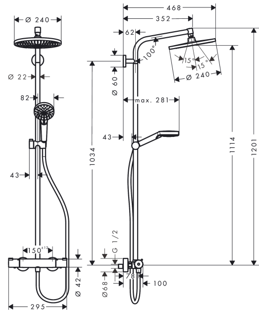
Scale drawing
