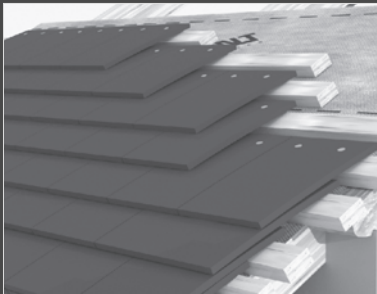
Conventional non-vented roof
