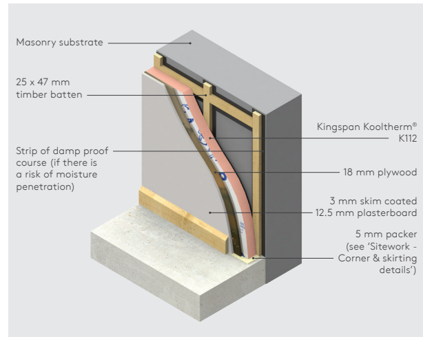
Figure 9: Mechanically fixed construction suitable for heavy internal fittings
