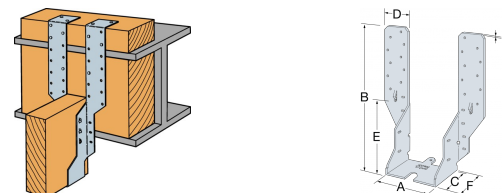
JHA450 Below Support Installation.
