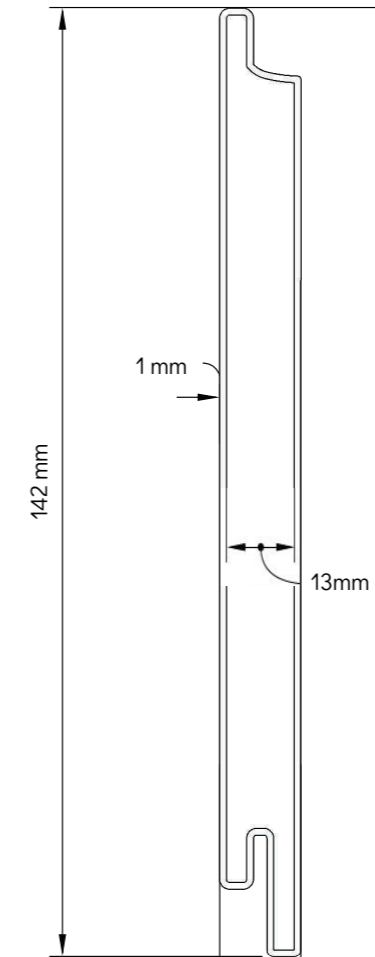
Panel cladding board dimensions
