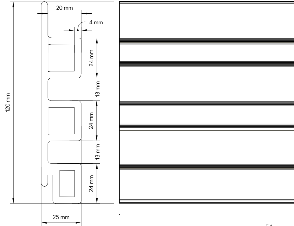
Slatted cladding board dimensions
