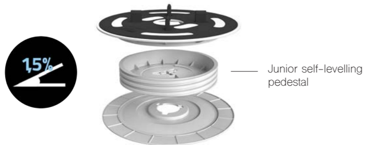
Junior Paving Pedestal J1 12mm - J3 30mm height
