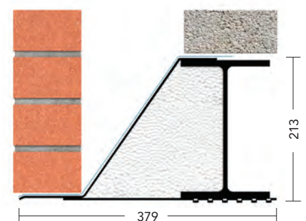
150-165mm cavity
