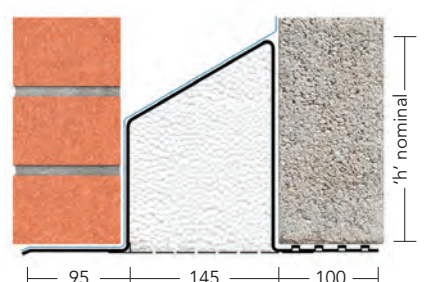
150-165mm cavity
