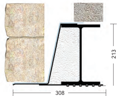
110-125mm cavity
