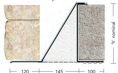
150-165mm cavity
