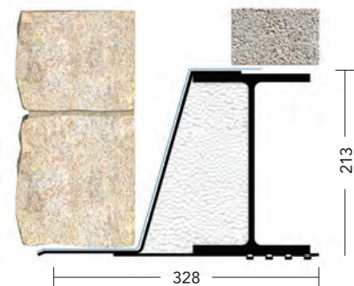
150-165mm cavity
