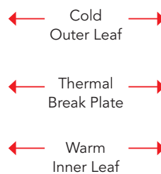
Standard IG Lintel with patented non-continuous Thermal Break Plate
