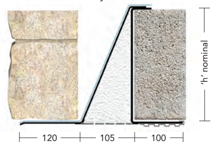
110-125mm cavity
