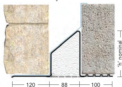
90-105mm cavity
