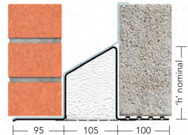
110-125mm cavity
