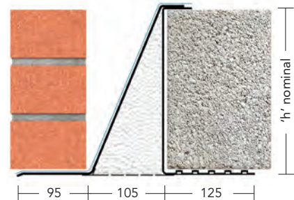
110-125mm cavity
