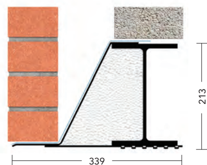
150-165mm cavity
