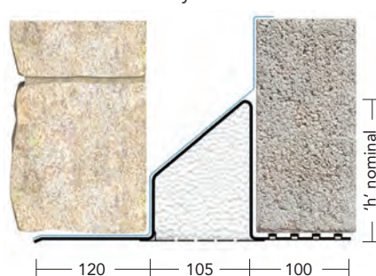
110-125mm cavity
