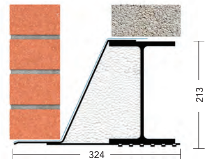
110-125mm cavity
