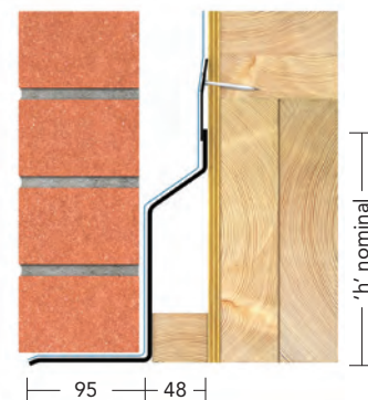
50-65mm cavity
