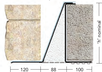
90-105mm cavity
