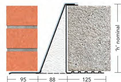
90-105mm cavity
