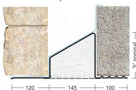
150-165mm cavity
