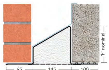
150-165mm cavity
