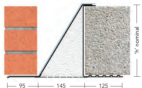
150-165mm cavity
