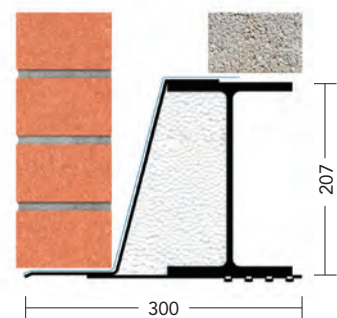
150-165mm cavity
