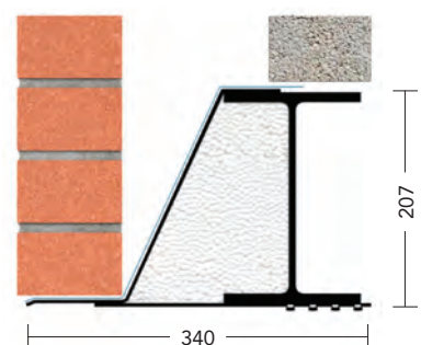
150-165mm cavity
