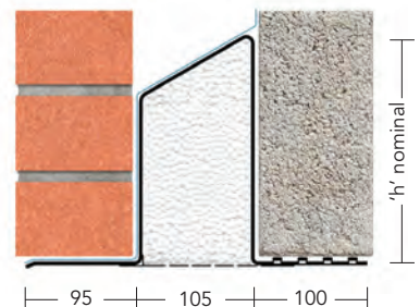
110-125mm cavity
