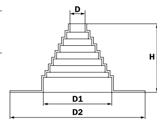
PIPE COLLARS
