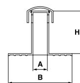
SINGLE WALL ROOF VENT
