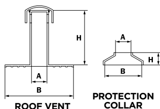
ROOF VENT
