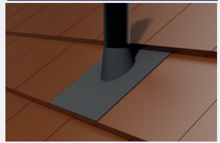
Pipe flashings
