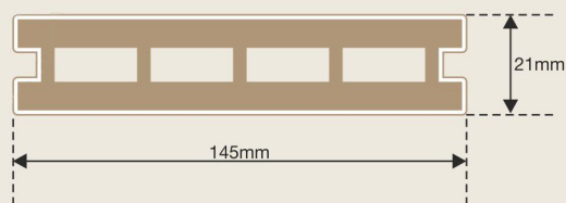
Board Dimensions: 145mm x 21mm
