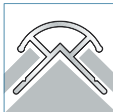
2 EXTERNAL CORNER To make an outside corner.
