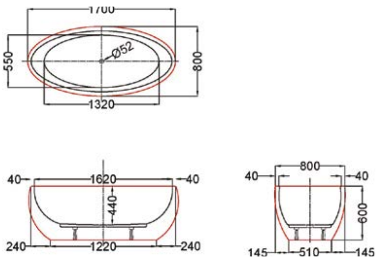
Sapporo Freestanding Bath
