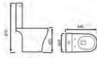
Comfort Height WC
