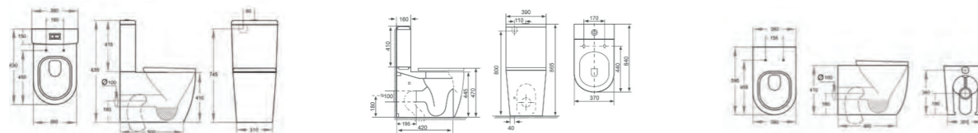
Close to Wall WC
