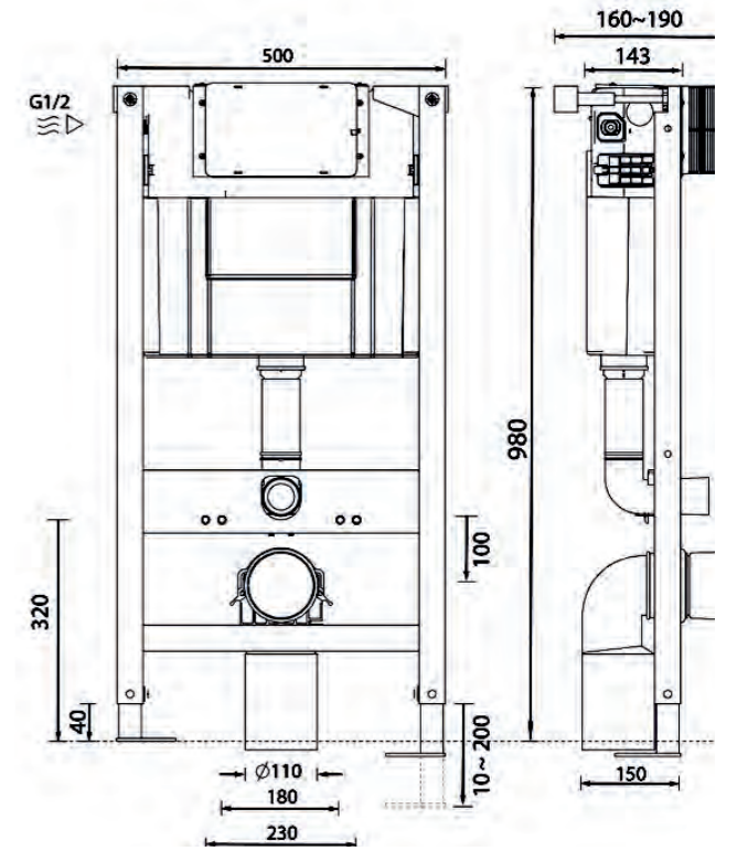
MODFR980 | 980mm
