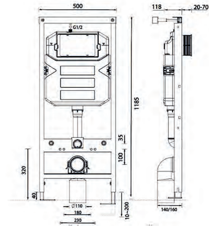
MODFR1180 | 1180mm
