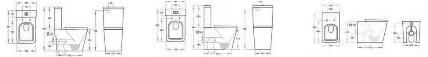
Close Coupled WC
