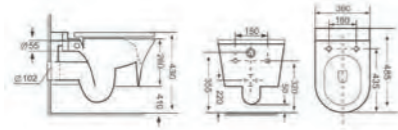
Wall Hung Pan
