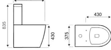
Close to Wall WC
