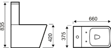
Close Coupled WC
