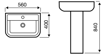
Basin with Pedestal
