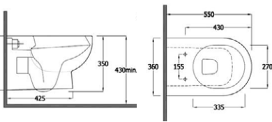
Wall Hung WC
