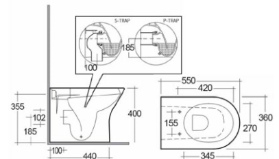
Back to Wall WC
