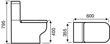
Close to Wall WC
