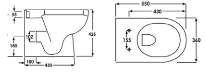
Back to Wall WC
