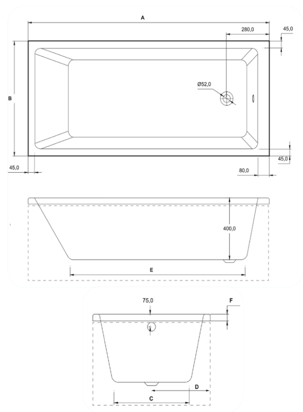
Single Ended
