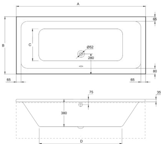
Double Ended
