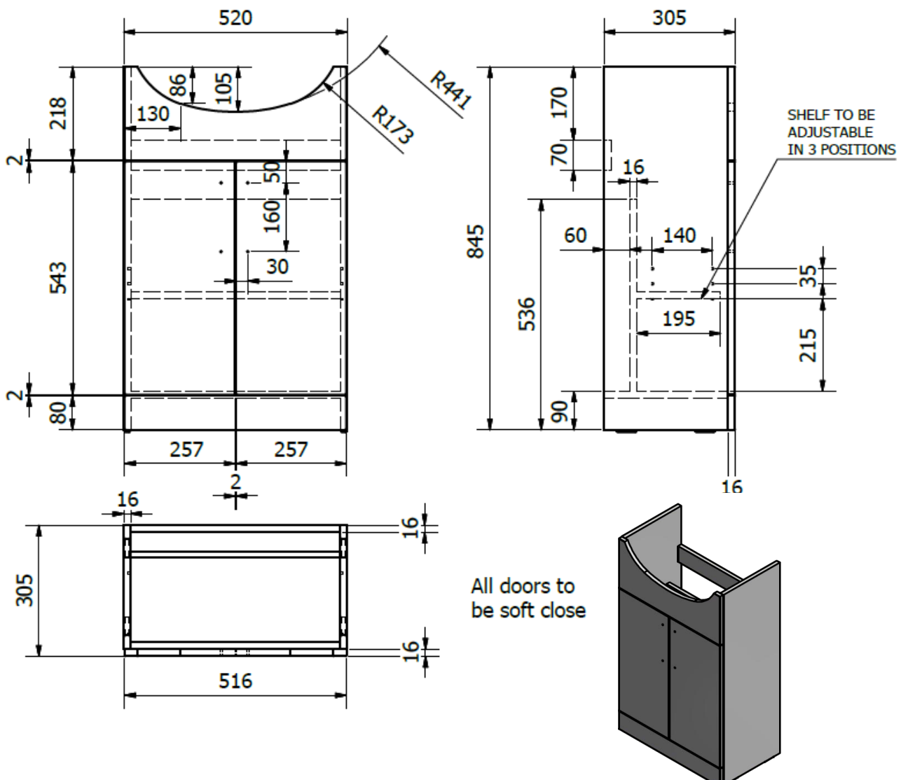
Technical drawing
