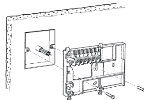
b. Flush switchbox Fixing holes are spaced to suit BS4662 requirements
