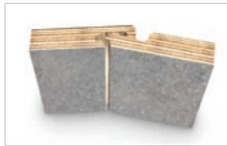
Fit 'grooved' edge first, and the 'tongued' edge of the next panel angled in
