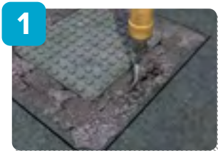
A picture frame is saw cut and excavated and the existing cover and frame removed.
