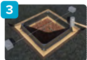
Apply UltraCrete bedding mortar (M60, M60 F, PY4 or Envirobéd® CD534) to the supporting structure and lower frame into position.
