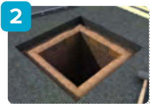
Old bedding mortar, loose bricks and debris are removed.
