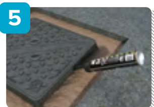
UltraCrete SCJ edge sealant and bitumen tack coat should be applied to all edges of the trim back and new frame.
