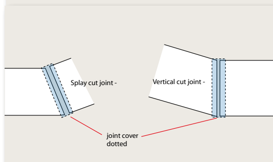
Fig. 23b Junction of fascia with In-line gable.
