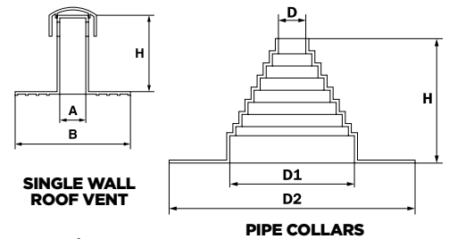
PIPE COLLARS
