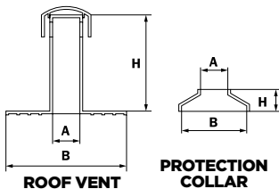
ROOF VENT
