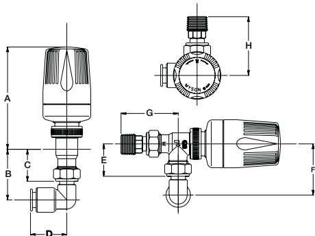
Description: Chrome Compression 90 TRV Size: 10mm Order Code: 2TRV10C90
