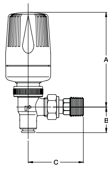
Description: Chrome Compression TRV Size: 10mm Order Code: 2TRV10C
