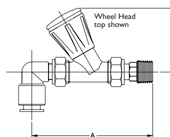
Description: Angle Chrome Compression 90 with Drain Off Lockshield Size: 10mm Order Code: MR10LACD90
