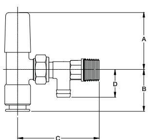
Description: Angle Chrome Compression 90 Lockshield Size: 10mm Order Code: MR10LAC90
