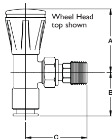
Description: Angle Chrome Compression 90 Lockshield Size: 10mm Order Code: MR10LAC90
