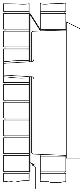
A polythene sheet 0.1mm thick or suitable cavity tray to be fitted by the builder
