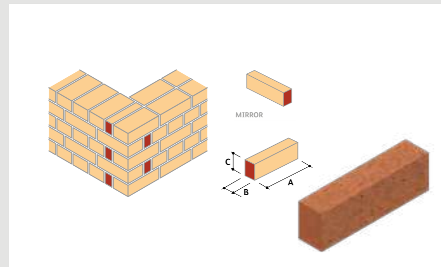
BD.3 Queen Closer
