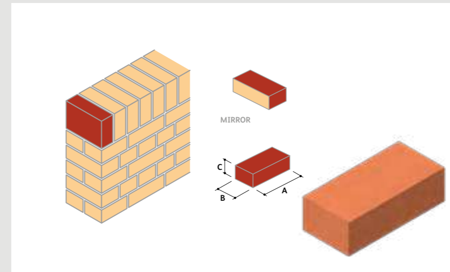
BD.1.3 Standard Brick fair-faced On Bed Surface
