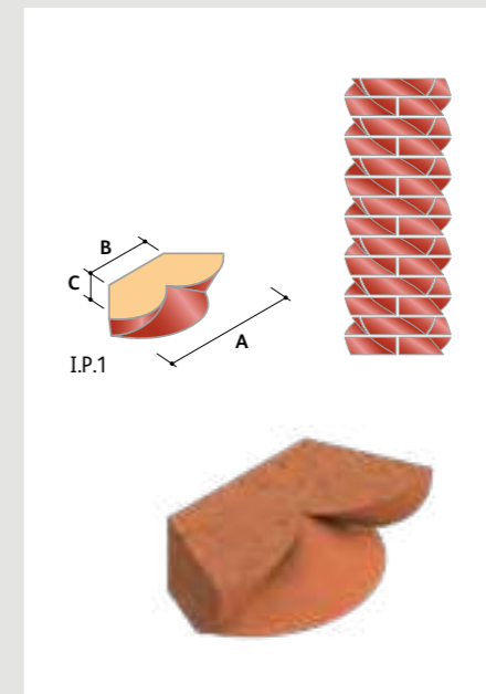
I.P.1 Pineapple Brick To 400mm Diameter Column
