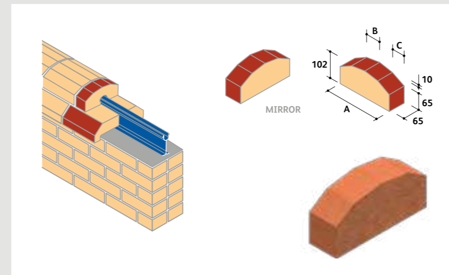
I.F.1 Faceted Capping +
