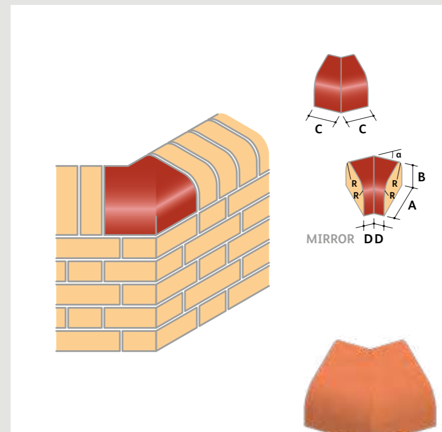
BN.21 Double Bullnose External Angle to Double Bullnose On Edge and to Bullnose Double Header On Flat
